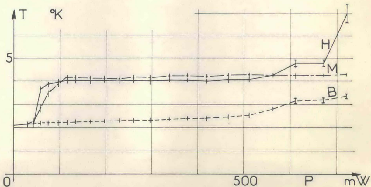
FIG.13 Superfluid helium T = 2.1 K ; p = 1 atm
