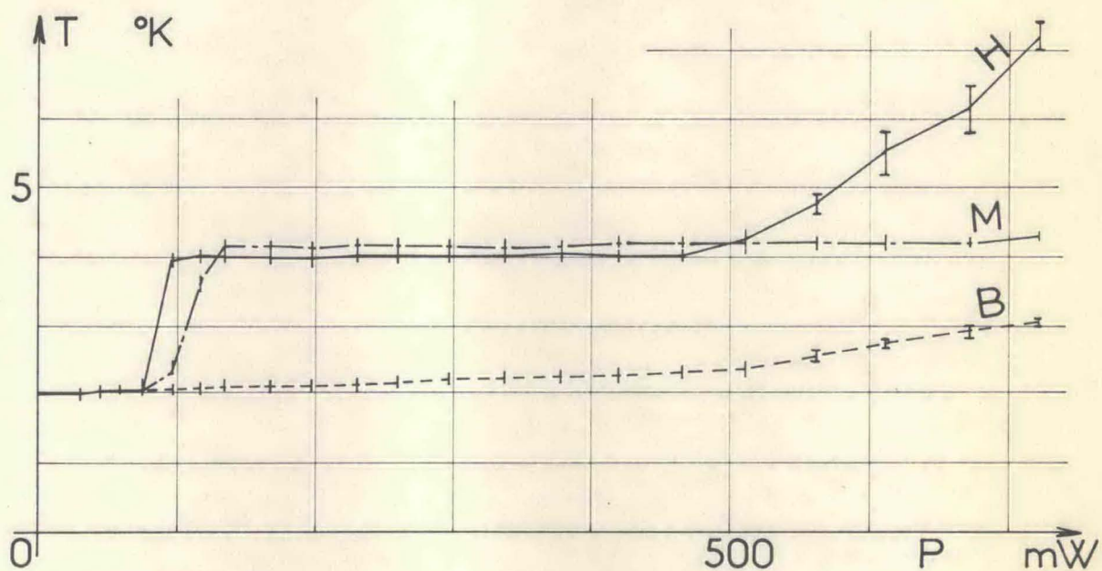
FIG.12 : Superfluid helium T = 2 K ; p = 1 atm
