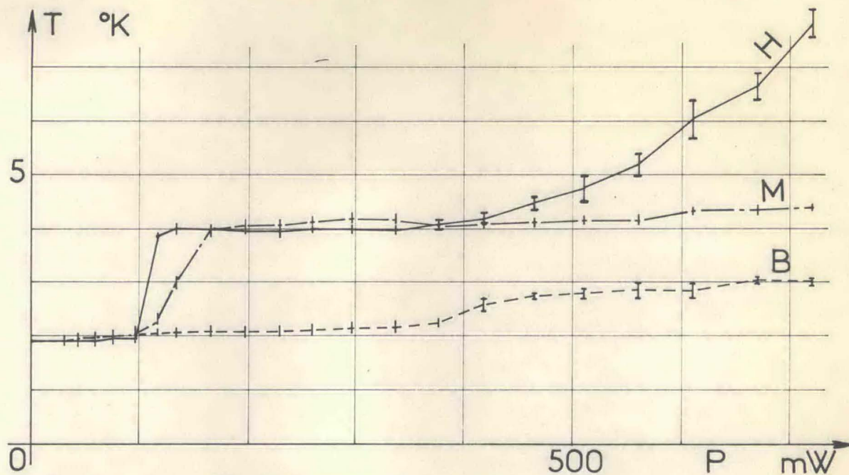
FIG.11 : Superfluid helium T = 1.9 K ; p = 1 atm
